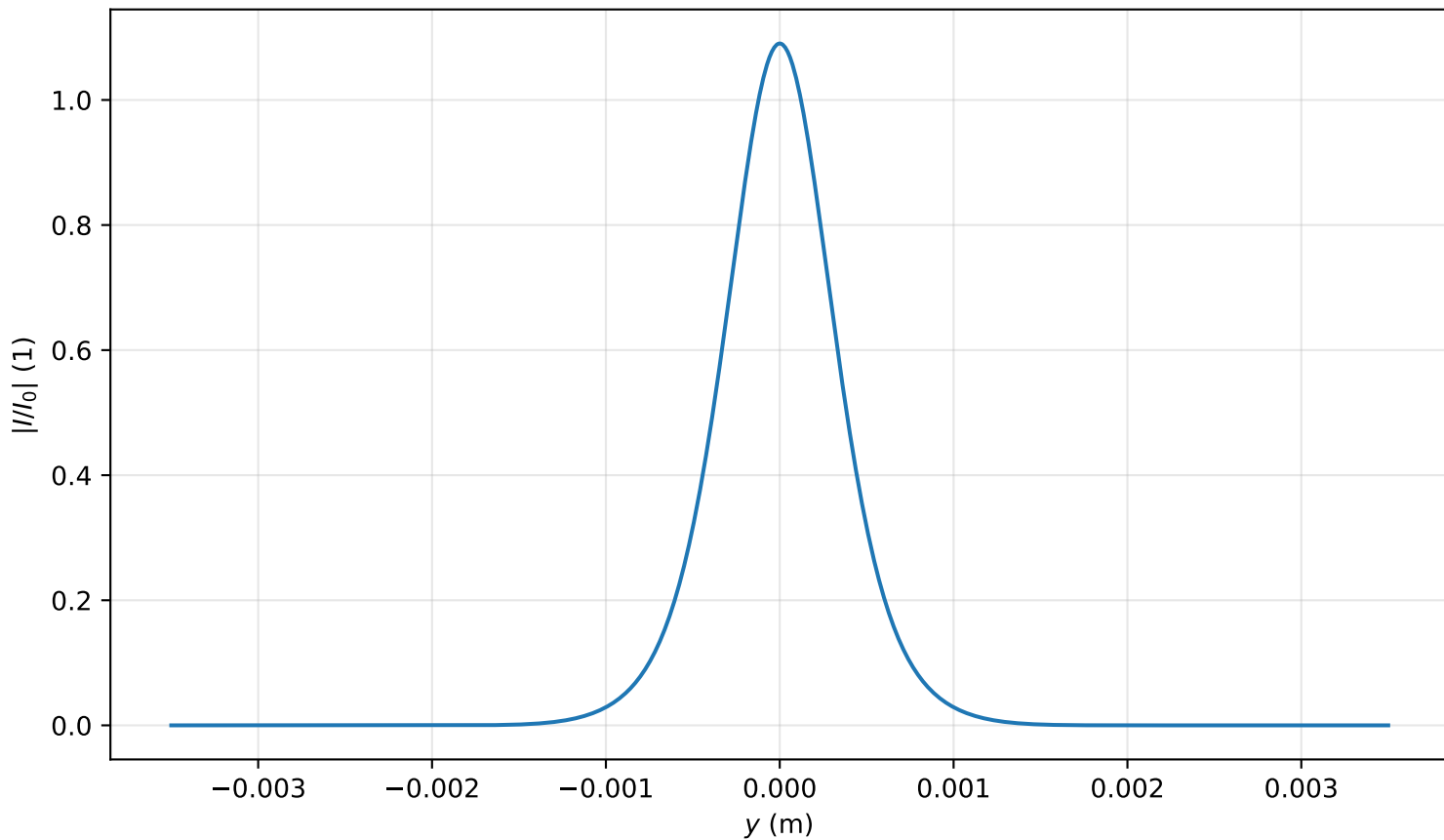
Intensity profile I(x = 0, y, z = 1.353)/I_0 , P_{in}=0.6P_{cr} , artificial time
